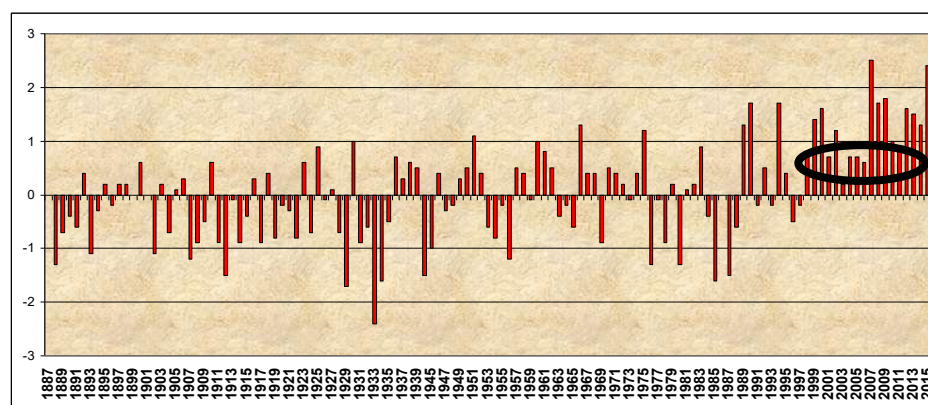
Fig.4. Annual thermic anomalies' evolution reported in the reference period of 1961- 1990
