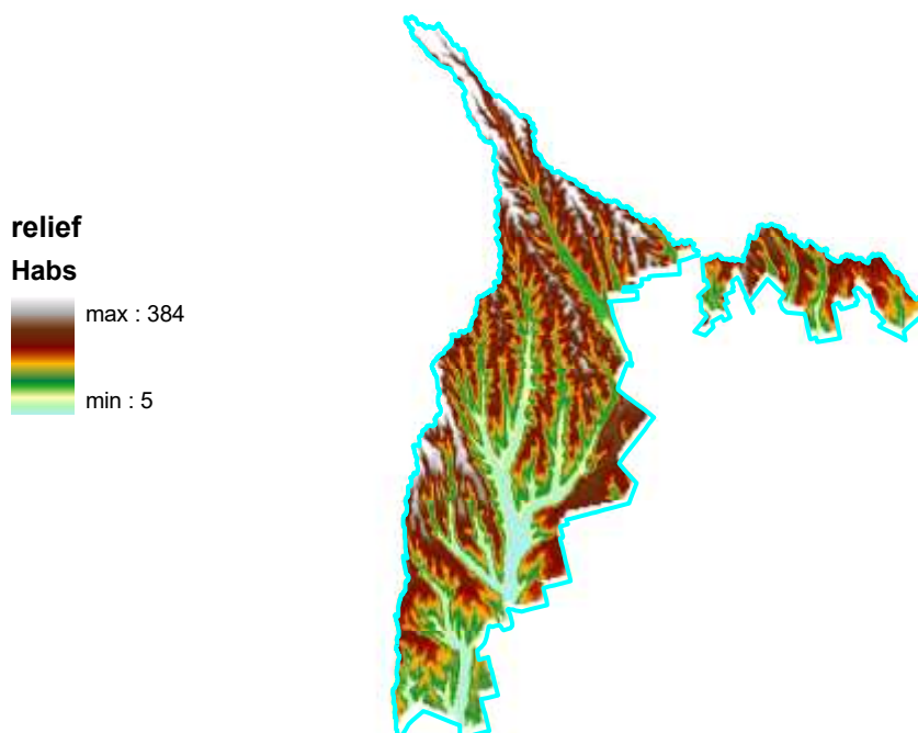
Fig.9. Absolute altitude map within the limits of Danube River's basin (Republic of Moldova)
